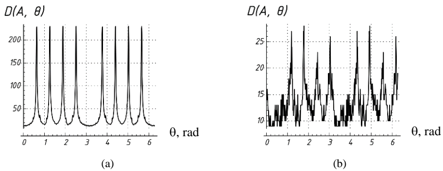
Fig. 3. Distributions of maxima in: (a) the accumulator of sample M_A ; (b) the accumulator of sample M_B
