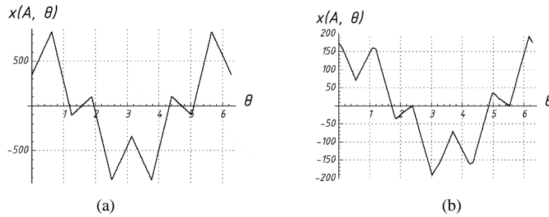
Fig. 7. Constructed asymmetry maps for accumulators of: (a) sample M_A ; (b) sample M_B
