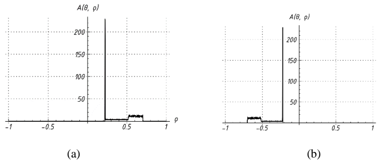
Fig. 6. Distribution of values in the columns of the accumulator matrix of Fig. 5 for: (a) A(\theta = 1.25) ; (b) A(\theta = 4.39)
