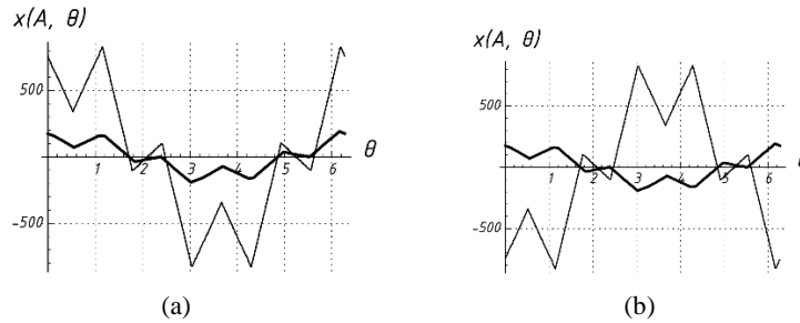
Fig. 8. Asymmetry maps shown in Fig. 7, with relative translations of: (a) \alpha = 0.52 ; (b) \alpha + \pi = 3.66
