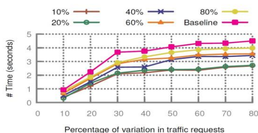
Fig. 5. Average times to re-allocate the service chains
